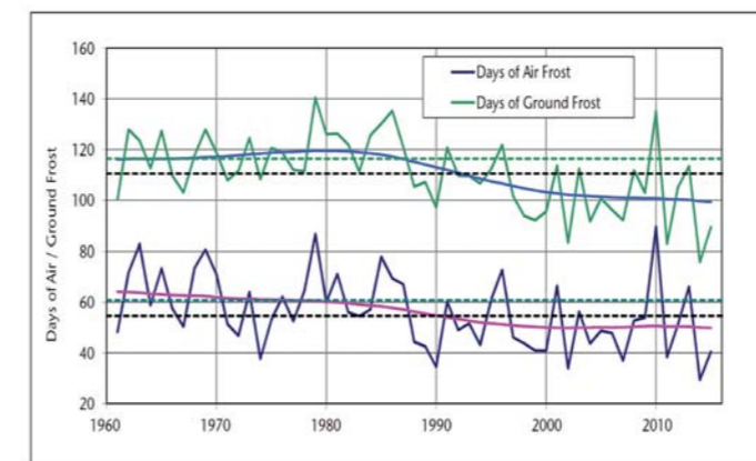
Figure 3.5: Annual number of days of air frost and ground frost for the UK, spanning from 1961 to 2015. The hatched black line represents the 1981 to 2010 annual average. Source: Kendon et al. 2016.
