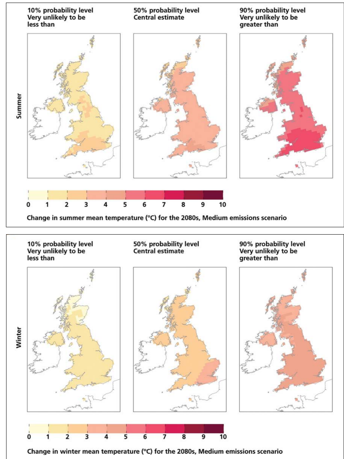
Figure 3.8: Projected changes in average temperature by the 2080s for summer (Top) and winter (Bottom) in °C for the medium emission scenario. Left, centre, right panels show: 10% probability, 50% probability and 90% probability respectively. Predictions are relative to the 1961–1990 baseline. Source: Jenkins et al. 2009.
