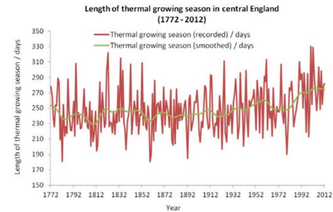
Figure 6.1: Growing season in Central England from 1772 to 2012 (red line). The green line shows data that have been smoothed to emphasise decadal timescale changes. Source: DECC 2013.
