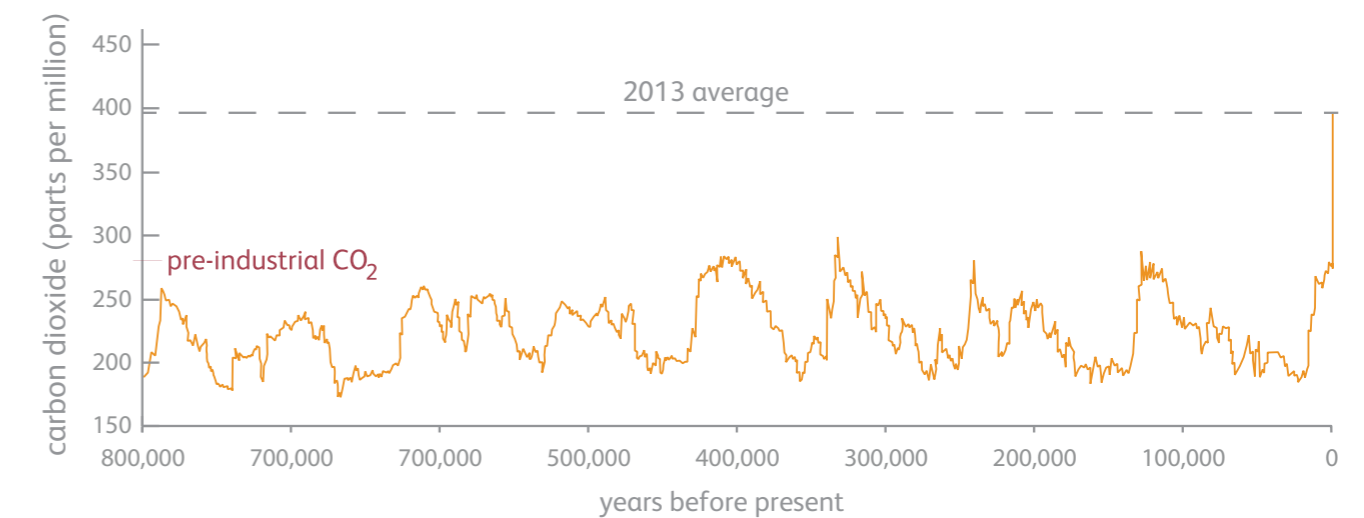
Figure 2.6: Atmospheric carbon dioxide concentrations in parts per million for the past 800,000 years, with the 2013 annual average concentration as a dashed line. The peaks and troughs in carbon dioxide levels follow the coming and going of ice ages (low CO 2 ) and warmer inter-glacial periods (higher CO 2 ). Source: Graph by NOAA Climate.gov, based on data from Lüthi et al. (2008), provided by NOAA NCDC Paleoclimatology Program (Blunden 2014).
