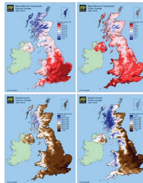
Figure 3.1: Clockwise from top left – average (mean) summer maximum air temperature (°C), average (mean) winter maximum air temperature (°C), and average winter rainfall (mm), average summer rainfall (mm). Averages refer to the period 1981–2010. Source: Met Office (2016).
