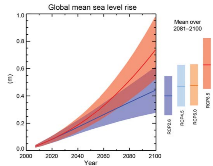
Figure 2.11: Projections of global mean sea level rise over the 21st century relative to 1986–2005 from a combination of several models. The range of the mean output from the models over the period 2081–2100 are given as coloured vertical bars. Source: IPCC (2013).
