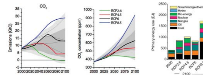
Figure 2.8: (Left) Emissions of CO 2 across RCPs, (Middle) trends in concentrations of CO 2 . Grey represents the area of uncertainty, dotted lines are an artefact of the baseline scenarios used in the calculation of RCPs. (Right) Energy sources by sector. Source: van Vuuren et al. (2011).
