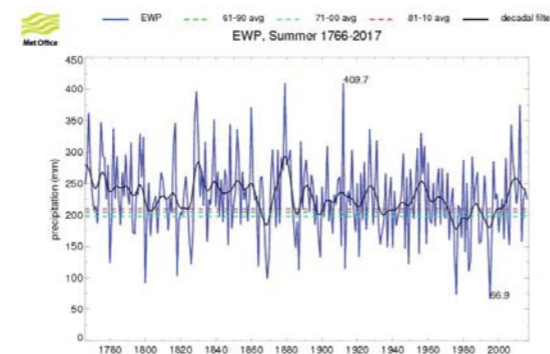
Figure 3.4: Precipitation (mm) in England and Wales during winter (December, January, February) (Top) and summer (June, July, August) (Bottom). The black line highlights decadal timescale variations from 1780 to 2017. The average England/Wales precipitation for 1961 to 1990, 1971 to 2000 and 1981 to 2010 is shown by the green, blue and pink dashed lines respectively (Met Office 2016b).
