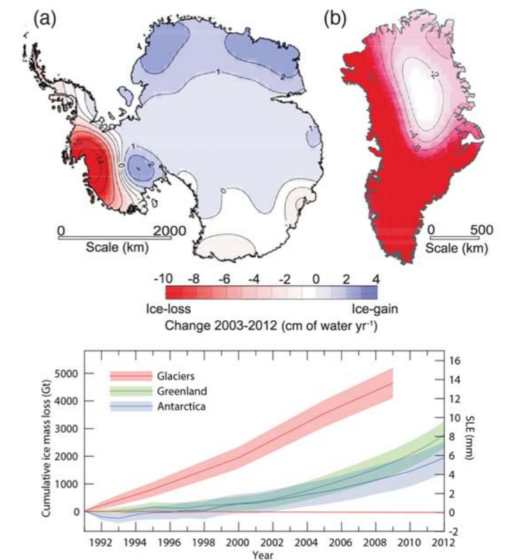
Figure 2.3: (Top panel) Ice loss/gain from (a) Antarctica and (b) Greenland, shown in centimetres of water per year for the period 2003–2012. (Bottom panel) The assessment of the total loss of ice from glaciers and ice sheets in terms of mass (Gt) and sea level equivalent (mm). The contribution from glaciers excludes those on the periphery of the ice sheets. Source: Stocker et al. (2013).
