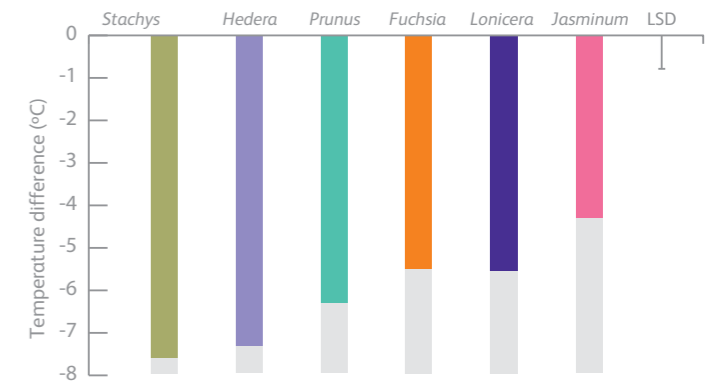
Figure 7.2: The extent to which different plant species can provide cooling to a building wall. The use of plant screens can reduce the amount of solar irradiance impacting on a building, thus reducing the requirement for artificial air conditioning. Comparison of a range of wall shrubs/ climbers with Stachys as a comparison (Cameron et al. 2014).
