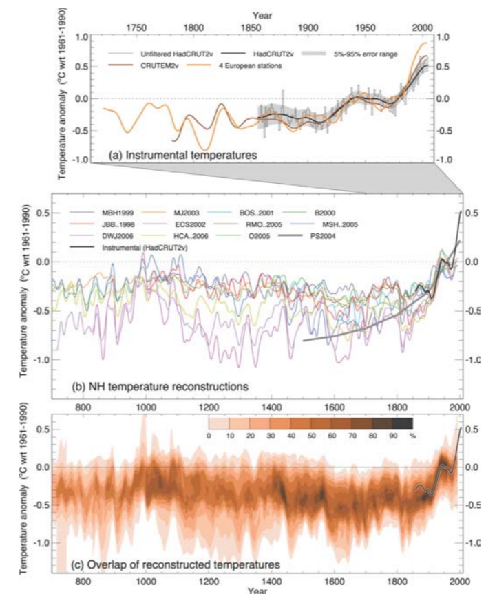
Figure 2.2: Northern Hemisphere temperature variation: (Top panel) over the period with direct instrumental records from thermometers, (Middle panel) since 700 AD reconstructed from multiple climate proxy records (derived from sources such as tree rings and corals) and (Bottom panel) the agreement between different proxy records. The orange shades indicate the level of agreement (darker colours indicate higher agreement). The instrumental temperature record is shown in black. All series have been smoothed to remove fluctuations on time scales less than 30 years. All temperatures represent anomalies (°C) from the 1961 to 1990 mean. Source: Jansen et al. (2007).
