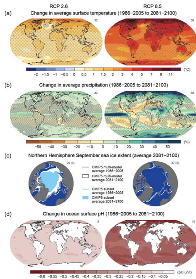
Figure 2.10: Maps showing the results generated from multiple model outputs. Changes are relative to the period 1986–2005. (a) Annual mean surface temperature change, (b) average per cent change in mean annual precipitation, (c) projection for Northern Hemisphere September sea ice extent (trend of the Arctic sea ice extent is given in light blue colour) and (d) change in ocean surface pH. Source: (IPCC 2013).
