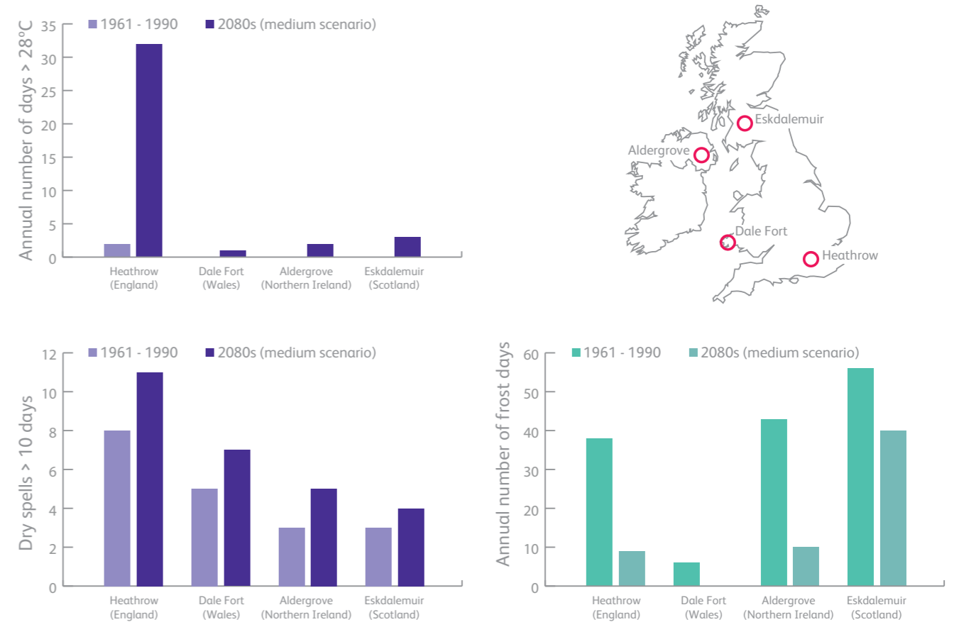
Figure 3.10: Clockwise from top left: annual number of days exceeding 28°C, map of locations of weather generator stations, annual number of days of air frost (days when minimum air temperature less than 0°C) and number of dry spells (defined as a single period longer than 10 days) over the course of a year. Results refer to the medium emissions scenario at the 50% probability level, based on 100 runs of the Weather Generator to a random sample of the projections. Raw data obtained from Jenkins et al. (2009).
