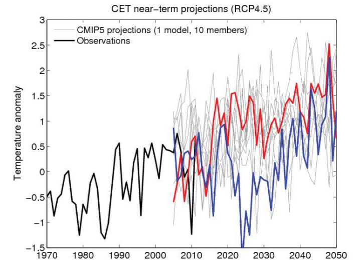
Figure 3.13: Central England Temperature from ten simulations of future climate (grey lines), with two simulations highlighted in red and blue. Source: Hawkins (2014).
