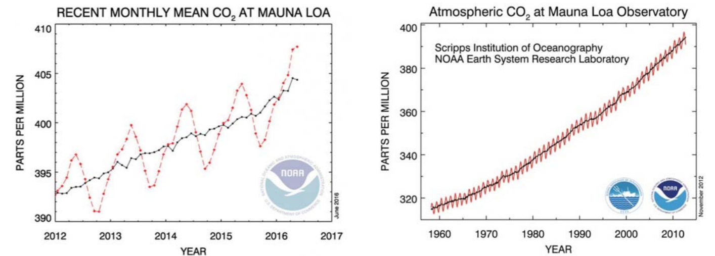
Figure 2.5: (Left) Recent monthly mean atmospheric CO 2 concentration at Mauna Loa for 2012 to 2016. Dashed red line indicates mean monthly values and the black line is the overall trend. (Right) Monthly mean CO 2 for Mauna Loa since the start of recording in 1958. Red and black lines same as for previous image. Source: National Oceanic and Atmospheric Administration (2016).
