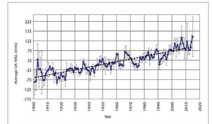
Figure 3.7: UK sea level rise since 1901 computed from sea level data from five stations (Aberdeen, North Shields, Sheerness, Newlyn and Liverpool). The black-hashed line indicates the linear trend of 1.4 mm per year. Error bars represent the uncertainty for each individual year (Kendon et al. 2016).
