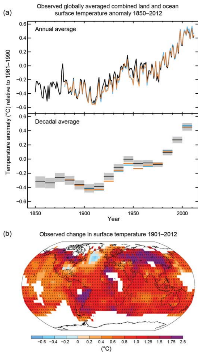
Figure 2.1: (a) Observed global mean surface temperature over the period 1850–2012 expressed relative to mean temperatures over the period 1961–90. Upper panel shows annual mean values (from three different temperature datasets) and lower panel shows decadal mean values with estimated uncertainty (grey shading). (b) Map of observed surface temperature change from 1901 to 2012. Source: IPCC (2013).
