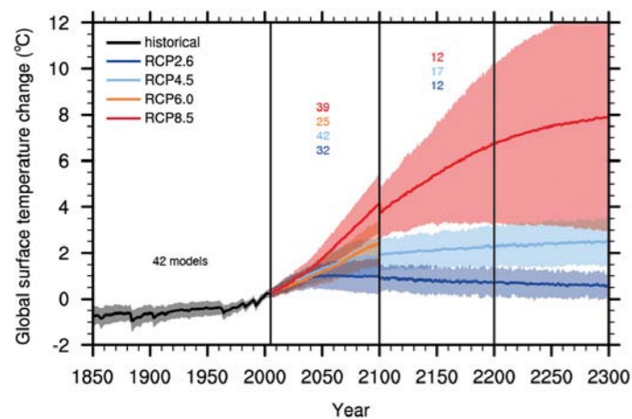
Figure 2.9: Time series of deviations in global annual mean surface air temperature (relative to 1986–2005). Solid lines represent the average (mean) of the output from multiple models, and the shading represents the range of model outputs. Discontinuities at 2100 are due to different numbers of models performing the runs beyond the 21st century and have no physical meaning. Source: Collins et al. (2013).
