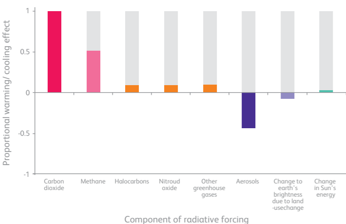
Figure 2.7: Proportional warming/cooling effect of increasing greenhouse gases, aerosols and changes in the Sun's energy since pre-industrial times. A positive value (red/orange) is a warming effect, and a negative value (blue) represents a cooling effect. Data adapted from Myhre et al., (2013).
