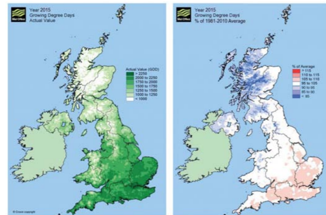
Figure 6.2: Number of Growing Degree Days in 2015 (Left) and percentage increase or decrease compared to the 1981 to 2010 average (Right). Source: (Kendon et al. 2016).
