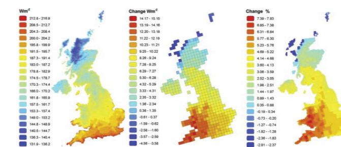
Figure 3.12: Summer solar resource: (left) baseline (1961–90); (middle) 2050s change in Watts per square meter ( Wm^{-2} ); and (right) percentage change from baseline. Source: Burnett et al.,
